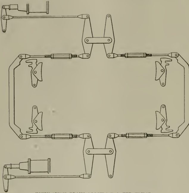
FOUNDATION BRAKE RIGGING FOR END TRUCK.
